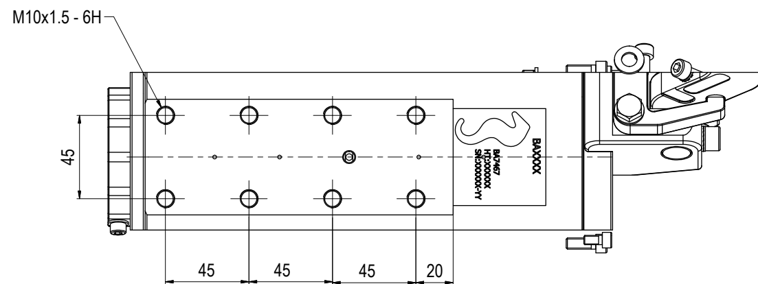
VIEW A-A (MOUNTING INTERFACE)
